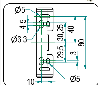
Attacco Anta Door Holder
