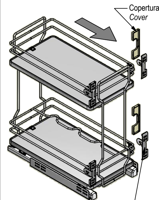
Attacco Anta Door Holder
